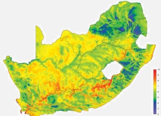
Wind Atlas of South Africa (WASA), Large Scale High Resolution Wind Resource map
